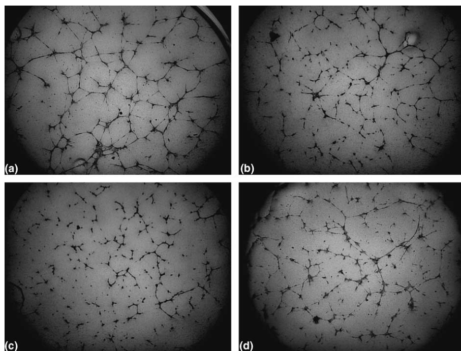
Figure 3. Effect of selected thioacetal artemisinin derivatives on tube formation by human umbilical vein endothelial cells (HUVEC) on Matrigel. (a) Control, (b) compound 8 (10 \mu\text{g/mL} ), (c) compound 11 (10 \mu\text{g/mL} ), (d) compound 16 (10 \mu\text{g/mL} ).
